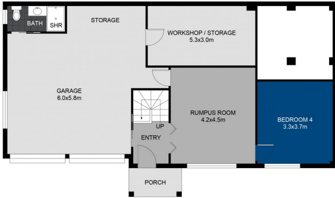
LOWER LEVEL FLOOR PLAN
